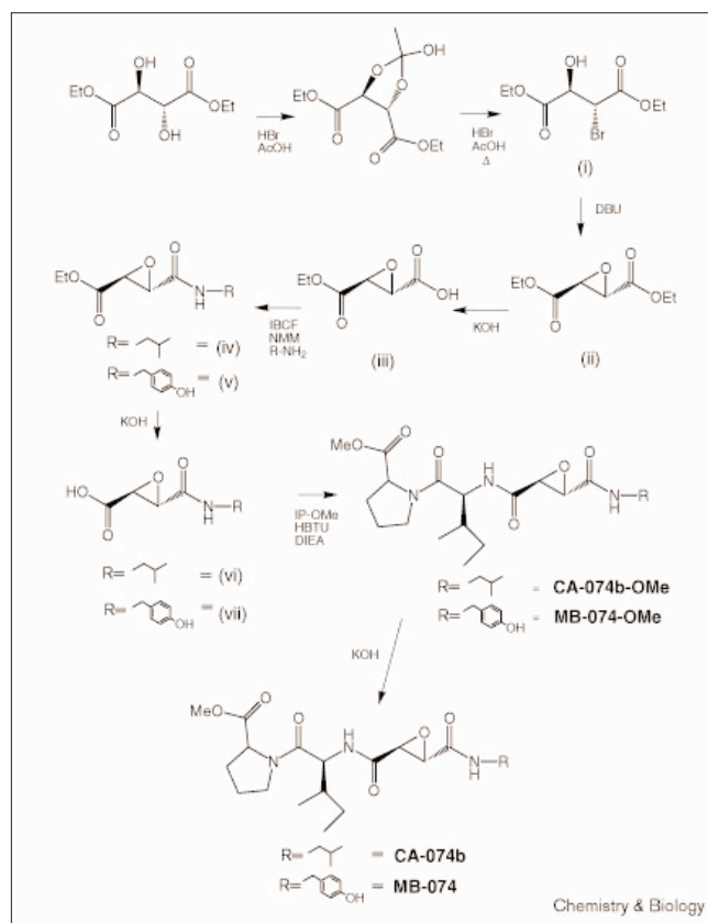
Synthesis of the peptide epoxides CA-074b-OMe, MB-074-OMe, CA-074b and MB-074.
